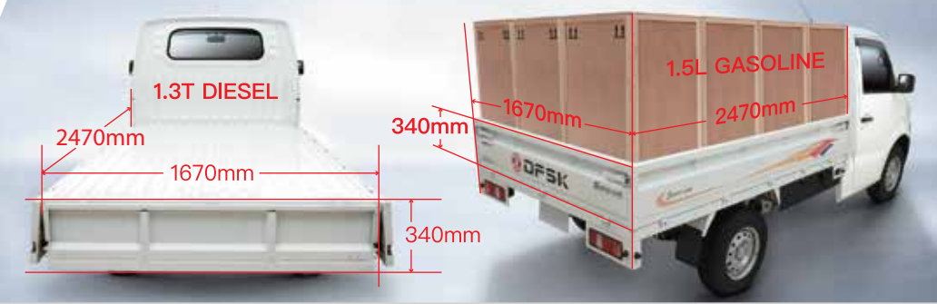
4-strip Cubical Support Rack with 16-pieces Cargo Bed Reinforcement Bars for a Longer Life Span
