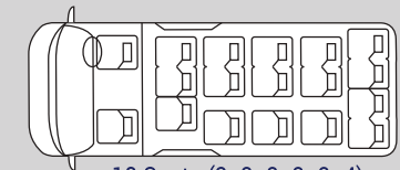
18 Seats (2+3+3+3+3+4)
